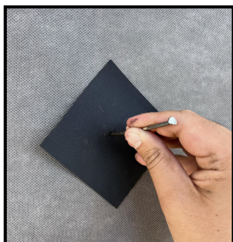
BLANK SEALS: Pierce blank FPS® Seal with a sharp point for each cable to pass through. Follow Step 2 & 3 above to ensure the seal is fitted correctly to the underlay.
