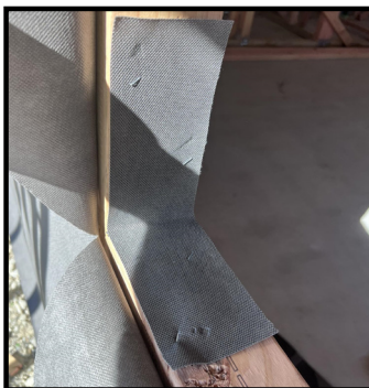
STEP 2: Insert section into corner of frame with equal length up and across frame. Fix in place with staples.
