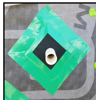
STEP 3: Remove the remaining section of backing paper and adhere to the FPS® underlay. Repeat for all other sides of the FPS® Seal, then firmly press tape with FPS® Spatula.
